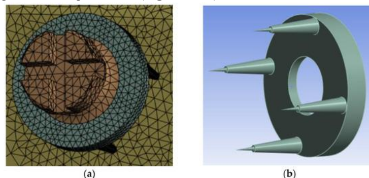
Figure 2. Stabilization Disc (SD) Configuration: The disc is flat with a central opening precisely aligned to the diameter of the mini-implant's neck. Its smooth surface is crafted from Ti6Al4V alloy, the same material as the implant itself
