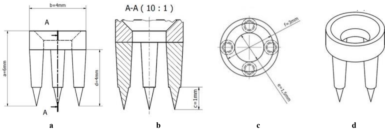
Figure 3. Detailed Representation of the SD: The illustration presents multiple views: (a) front elevation; (b) cross-section along line A–A; (c) plan view from above; (d) isometric perspective. Key dimensions are labeled as follows: ring height 6 mm (a), ring diameter 4 mm (b), maximum insertion depth 1 mm (c), leg height 4 mm (d), internal diameter 1.5 mm (e), and external diameter 3 mm (f)
