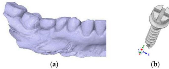
Figure 1. Finite Element Modeling Approach: (a) STL-format optical scan of the mandible; (b) STL-format CT scan of mini-implant model 1 and the corresponding CAD reconstruction produced in Spaceclaim
