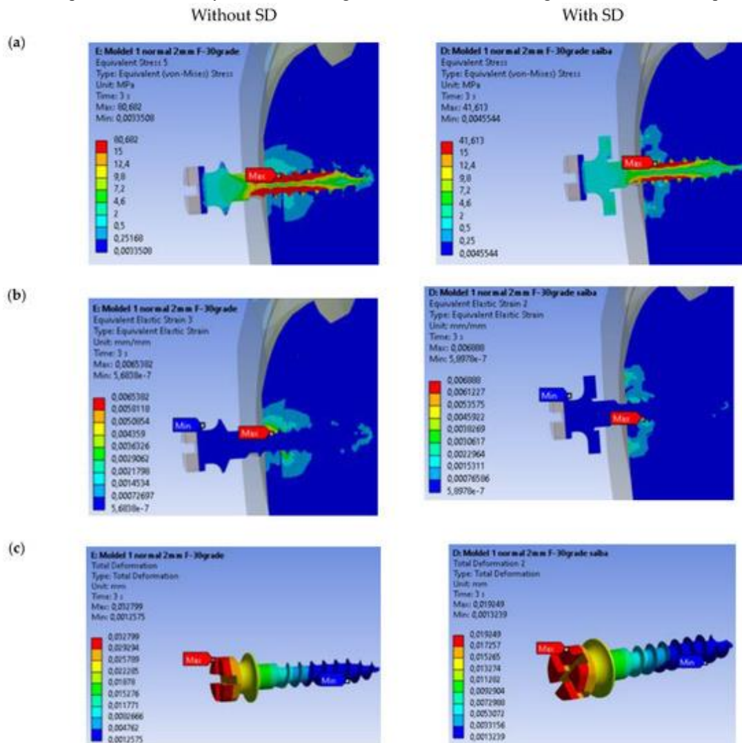
Figure 4. Comparative Evaluation: (a) Equivalent von Mises stresses; (b) linear equivalent strain distribution; (c) total deformation of the mini-implant, with and without the SD
